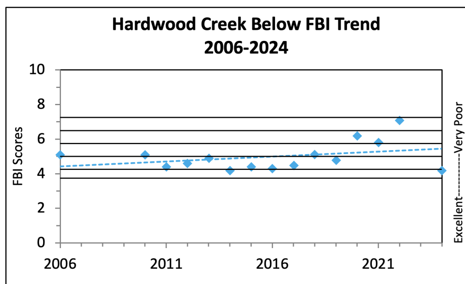
Figure 10. The graph is entitled “ Hardwood Creek Below FBI Trend 2006-2024”. The vertical axis, left side, is labeled “FBI Scores” beginning with zero and ending at ten, in increments of 2. The vertical axis, right side, is labeled “Excellent” on the lower end of the graph, and “very poor” at the higher end. The horizontal axis marks years from 2006 to 2024, in increments of 5. The trendline equation for this graph is y = 0.0567x + 4.3652 . A stream health trend was created using scores calculated for family biotic index (FBI). Contrary to common sense, a descending trendline indicates improvement in the stream health since organisms with sensitivity to water pollution score lower on the family biotic index.
